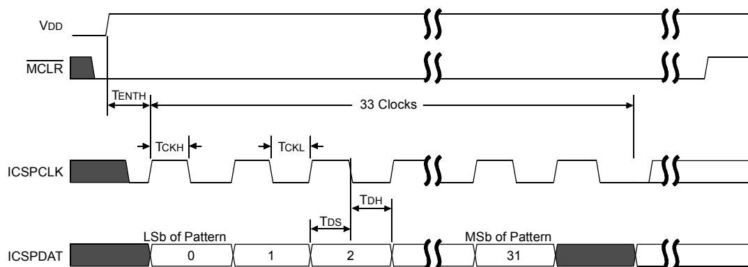
FIGURE 8-9: LVP ENTRY (POWERED)
