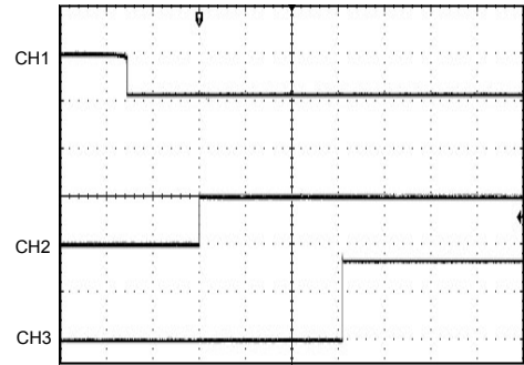
Startup of nPBIN, OUT6, nRSTO
