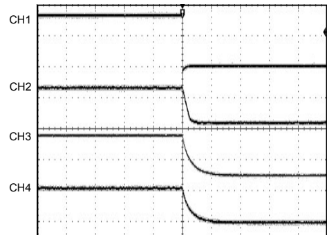
Sleep of PWREN, OUT4/2/3
