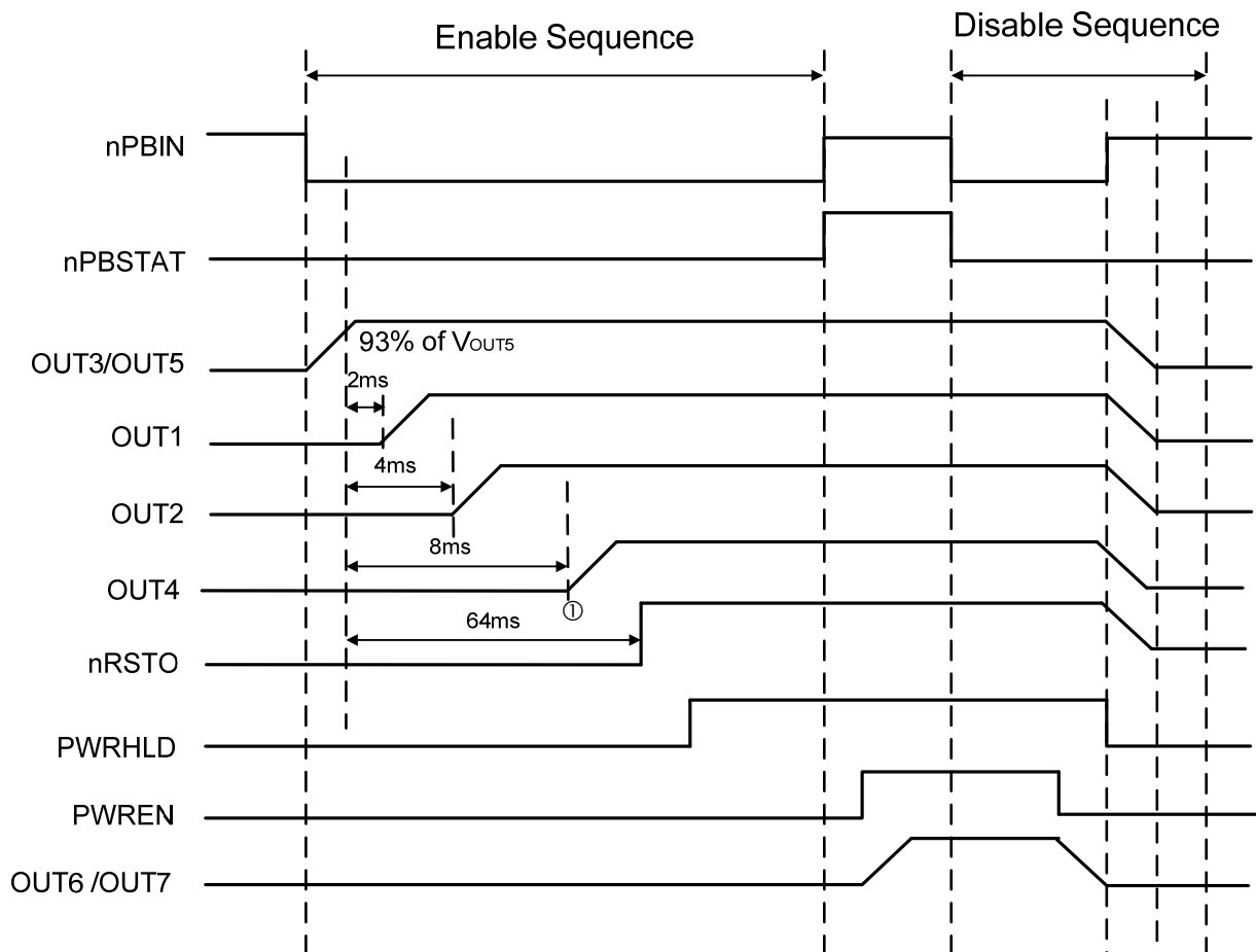
ACT8865QI305-T Enable/Disable Sequence
