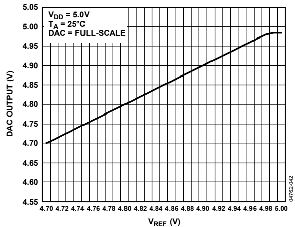
Figure 28. Typical Output Voltage vs. Reference Voltage
