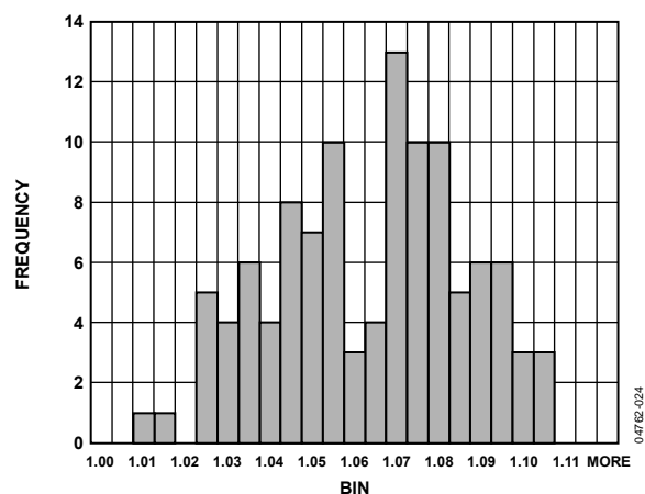
Figure 24. I_{DD} Histogram @ V_{DD} = 5\text{V}
