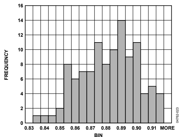
Figure 23. I_{DD} Histogram @ V_{DD} = 3\text{V}
