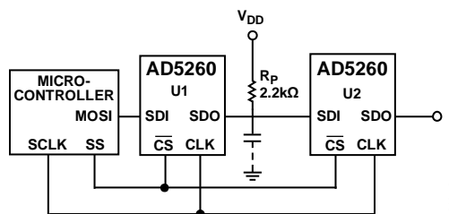
Figure 52. Daisy-Chain Configuration
