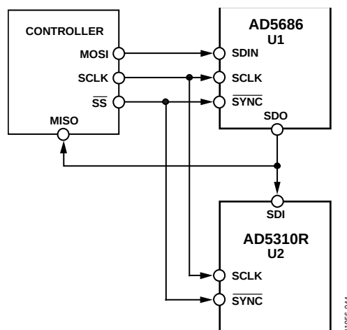
Figure 39. Daisy-Chain Connection
