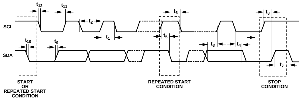
Figure 4. I²C Serial Interface Timing Diagram
