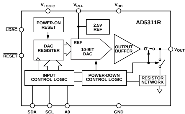
Figure 2. AD5311R
