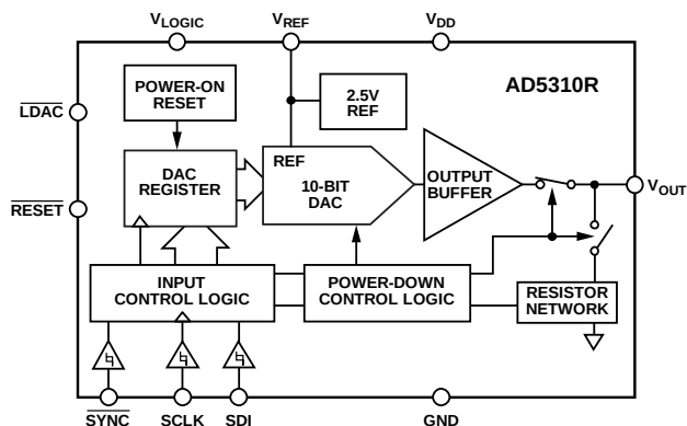
Figure 1. AD5310R
