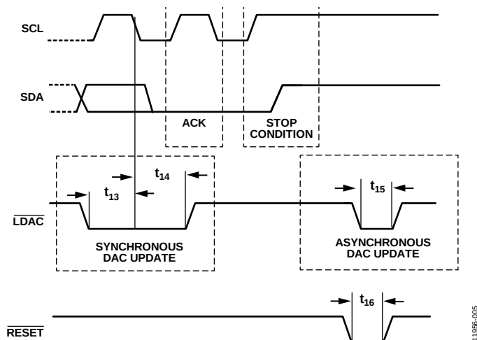
Figure 5. I 2 C, LDAC, and RESET Timing
