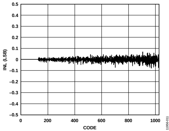
Figure 8. INL
