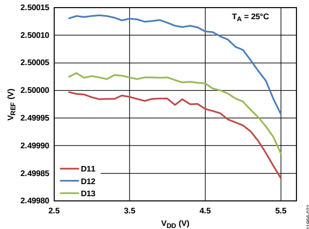
Figure 19. Internal Reference Voltage vs. Supply Voltage
