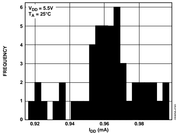
Figure 31. I_{DD} Histogram with Internal Reference, V_{REFOUT} = 2.5\text{ V}
