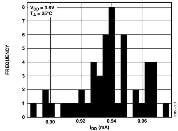
Figure 33. I_{DD} Histogram with Internal Reference, V_{REFOUT} = 1.25\text{ V}
