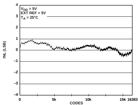
Figure 14. INL AD5648-2
