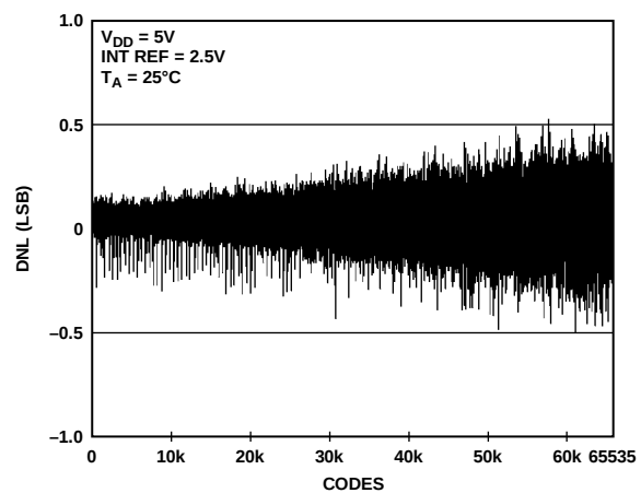
Figure 16. DNL AD5668-2/AD5668-3
