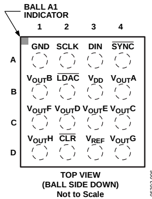
Figure 6. 16-Lead WLCSP
