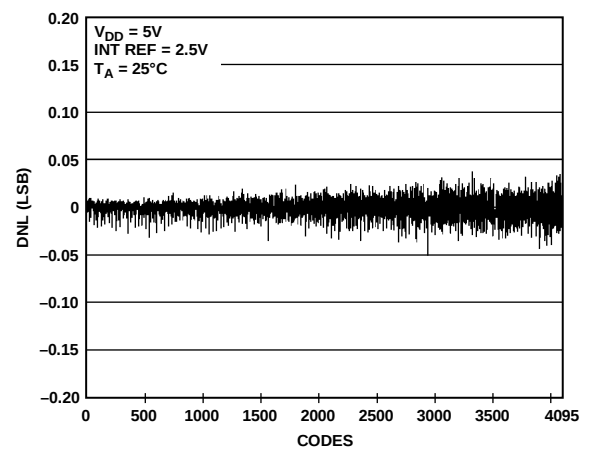
Figure 18. DNL AD5628-2
