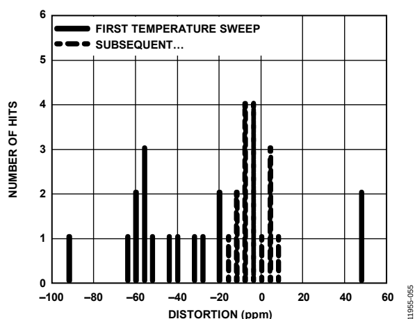
Figure 54. Thermal Hysteresis
