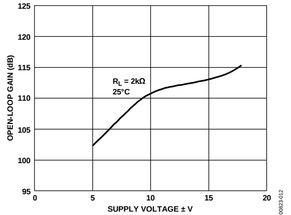
Figure 12. Open-Loop Gain vs. Supply Voltage
