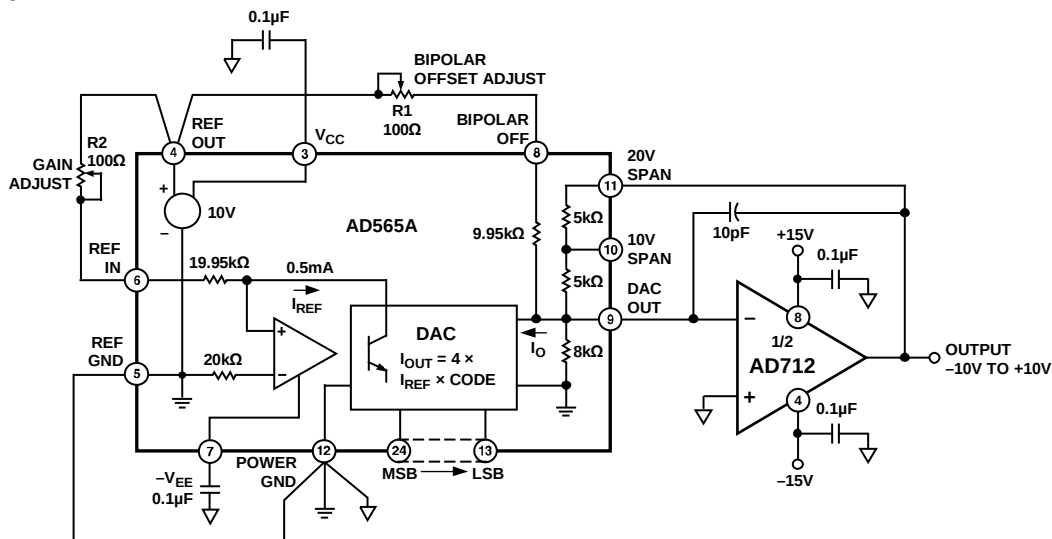
Figure 31. \pm 10\text{ V} Voltage Output Bipolar DAC
