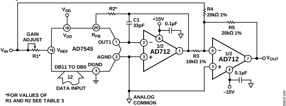
Figure 40. Bipolar Operation
