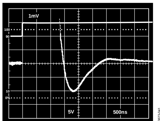
Figure 41. Positive Settling Characteristics for AD712 with AD7545
