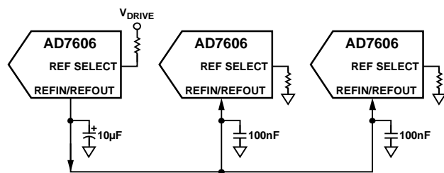
Figure 42. Internal Reference Driving Multiple AD7606/AD7606-6/AD7606-4 REFIN Pins
