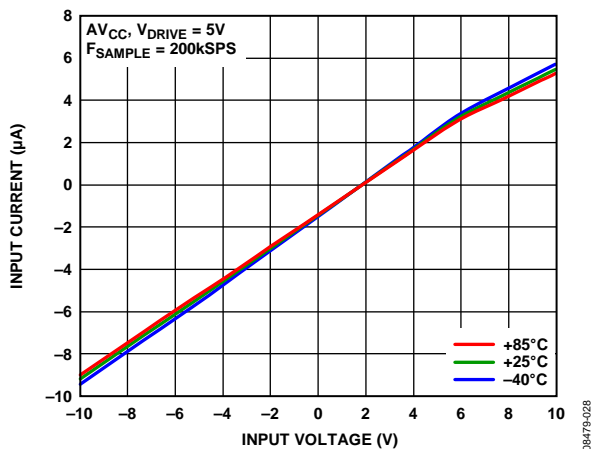
Figure 31. Analog Input Current vs. Temperature for Various Supply Voltages
