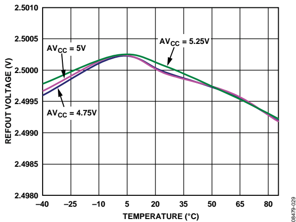
Figure 30. Reference Output Voltage vs. Temperature for Different Supply Voltages
