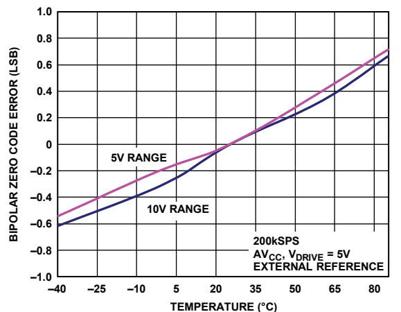
Figure 22. Bipolar Zero Code Error vs. Temperature
