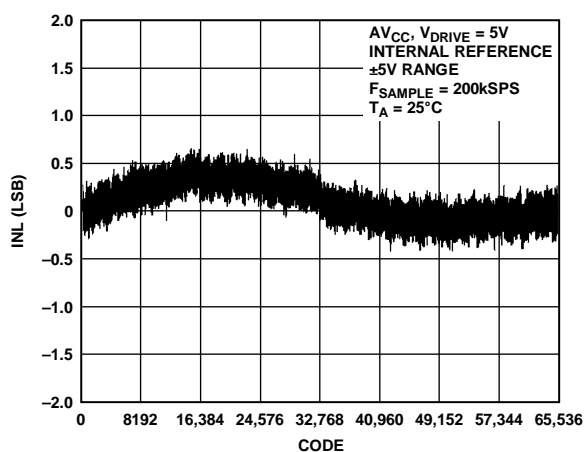
Figure 16. AD7606 Typical INL, ±5 V Range
