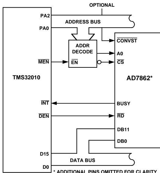
Figure 15. AD7862–TMS32010 Interface
