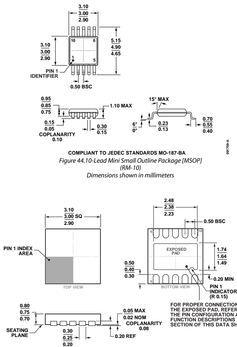
Figure 45. 10-Lead Lead Frame Chip Scale Package [LFCSP_WD] 3 mm × 3 mm Body, Very Very Thin, Dual Lead (CP-10-9)
