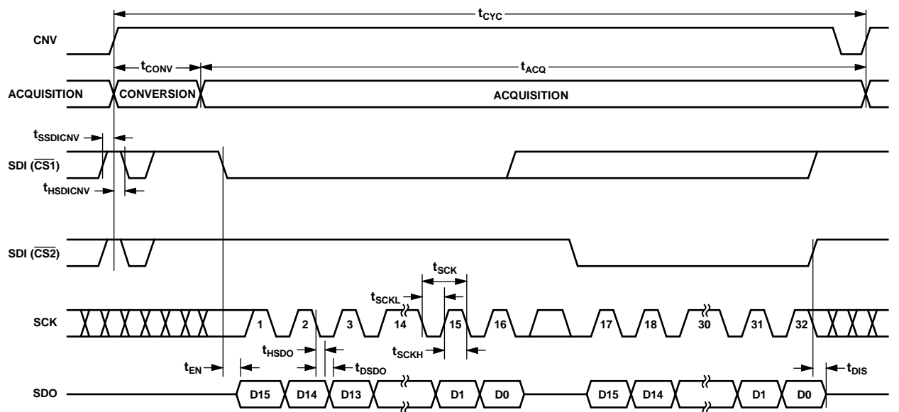
Figure 37. 4-Wire \overline{\text{CS}} Mode Serial Interface Timing
