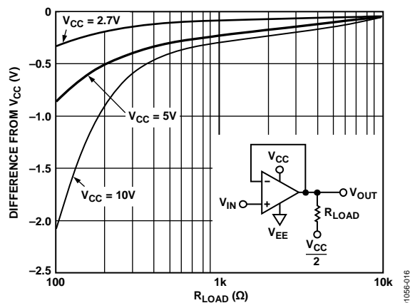
Figure 16. +Output Saturation Voltage vs. R_{LOAD} @ -40°C
