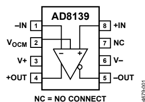
Figure 1. 8-Lead SOIC
