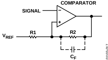
Figure 17. Configuring the AD8564 with Hysteresis
