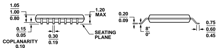
Figure 36. 14-Lead Thin Shrink Small Outline Package [TSSOP] (RU-14)
