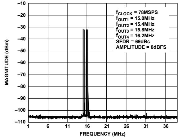
Figure 43. Four-Tone SFDR
