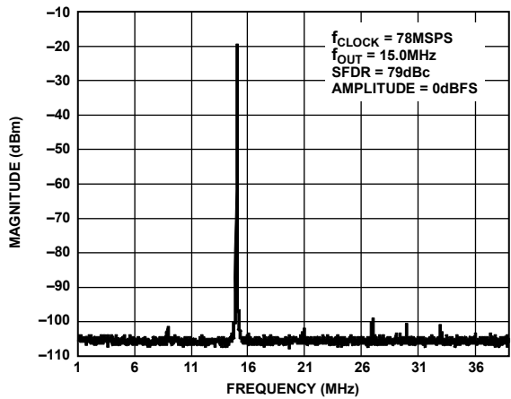
Figure 41. Single-Tone SFDR
