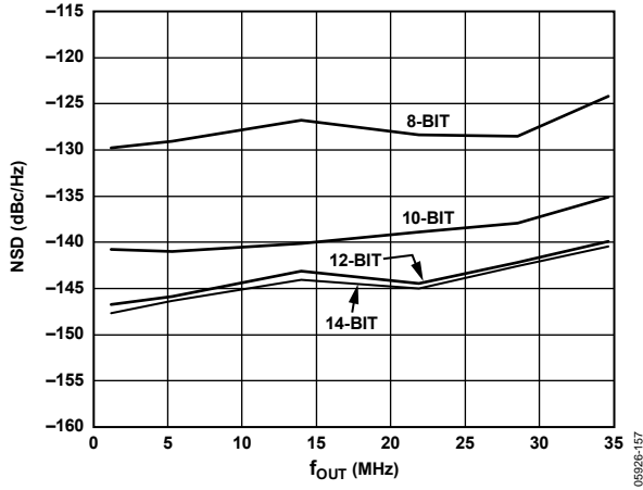
Figure 57. AD9704, AD9705, AD9706, AD9707 NSD vs. f_{out} at 0 dBFS, 80 MSPS
