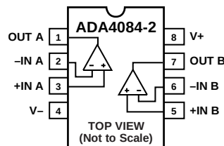
Figure 1. 8-Lead MSOP (RM), 8-Lead SOIC (R), 8-Lead LFCSP (CP)
