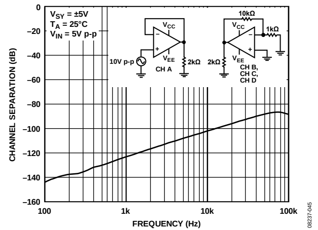
Figure 55. Channel Separation
