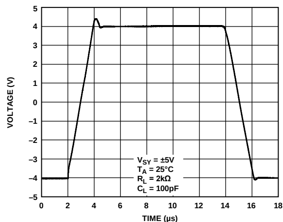
Figure 49. Large Signal Transient Response
