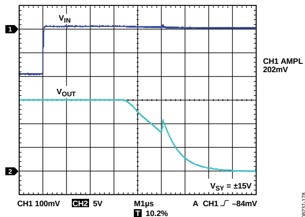
Figure 87. Positive Overload Recovery
