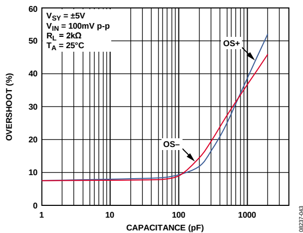
Figure 53. Overshoot vs. Load Capacitance
