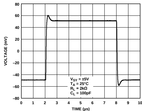
Figure 50. Small Signal Transient Response
