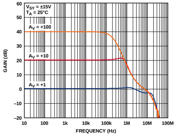
Figure 73. Closed-Loop Gain vs. Frequency
