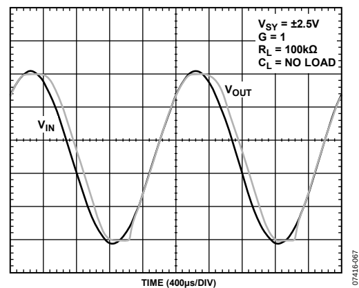
Figure 52. No Phase Reversal
