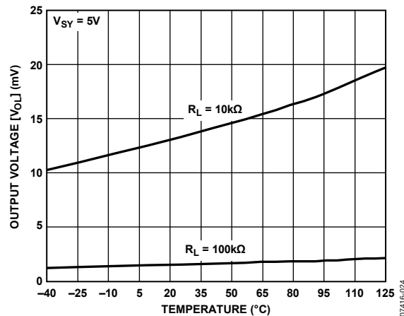
Figure 24. Output Voltage ( V_O ) vs. Temperature
