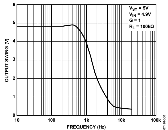
Figure 51. Output Swing vs. Frequency
