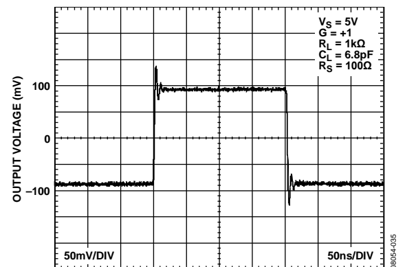
Figure 58. 200 mV Step Response, C_L = 6.8\text{ pF} , R_S = 100\text{ }\Omega
