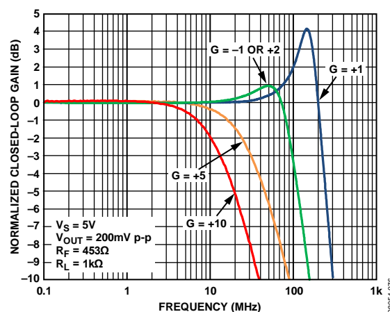
Figure 10. Small-Signal Frequency Response vs. Gain, V_S = 5V , ADA4891-3/ADA4891-4
