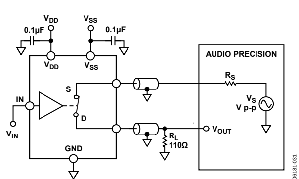
Figure 35. THD + Noise
