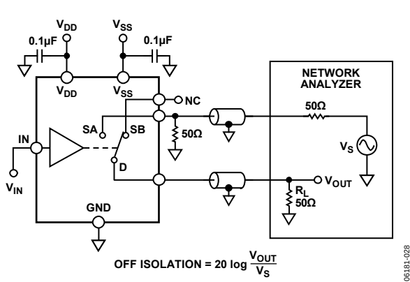
Figure 32. Off Isolation
