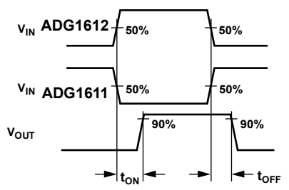
Figure 31. Switching Times
