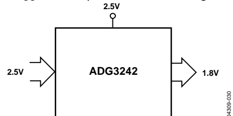
Figure 31. 2.5 V to 1.8 V Voltage Translation, \overline{SEL} = 2.5 V
