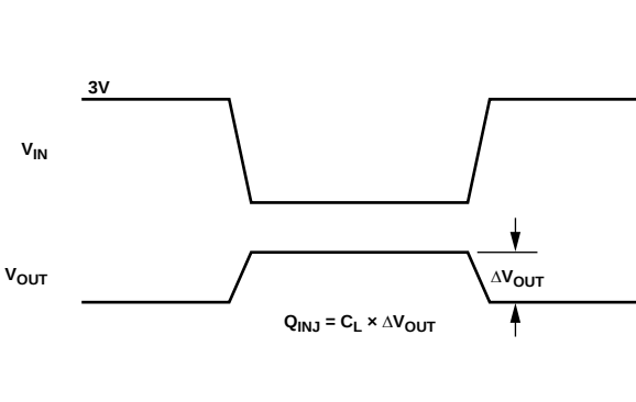
Figure 18. Charge Injection
