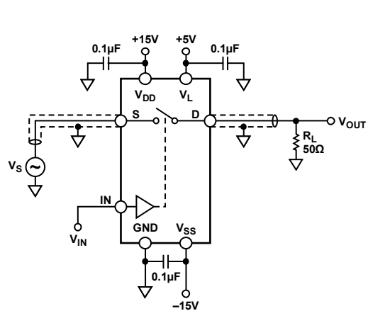
Figure 22. Off Isolation
