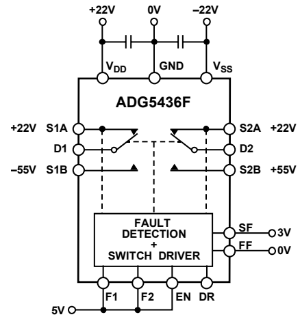
Figure 50. ADG5436F Under Example Overvoltage Conditions
