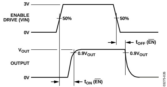
Figure 26. Enable Delay, t_{ON}(\overline{EN}) , t_{OFF}(\overline{EN})
