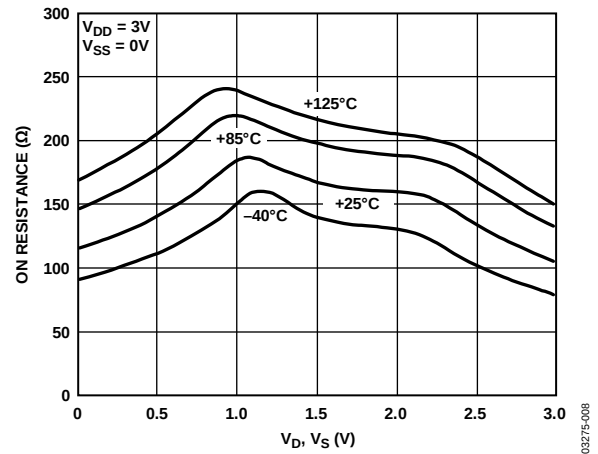
Figure 8. On Resistance vs. V_D ( V_S ) for Various Temperatures, Single Supply
