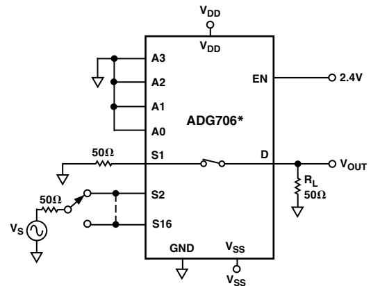
Test Circuit 10. Channel-to-Channel Crosstalk
