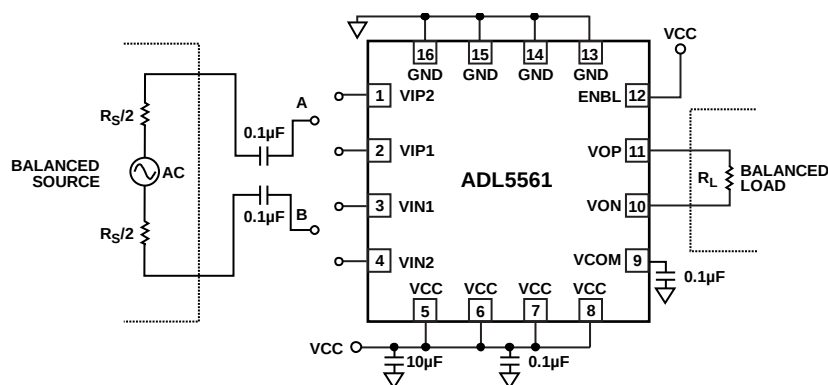
Figure 33. Basic Connections
