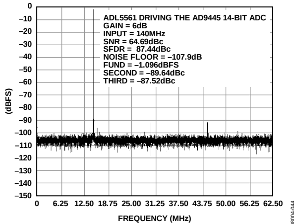
Figure 40. Measured Single-Tone Performance of the Circuit in Figure 39 for a 140 MHz Input Signal
