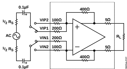
Figure 32. Basic Structure
