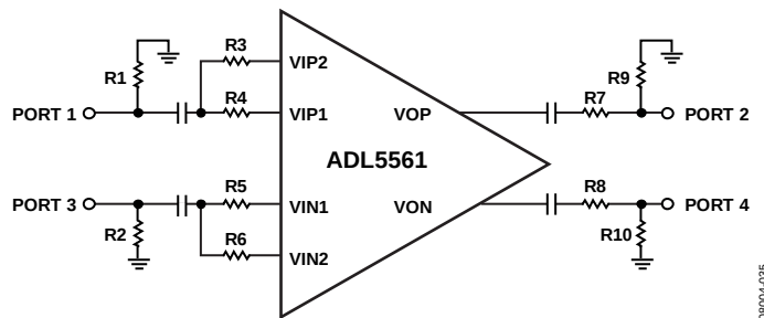
Figure 44. Differential Characterization Circuit Using Agilent E8357A 4-Port PNA
