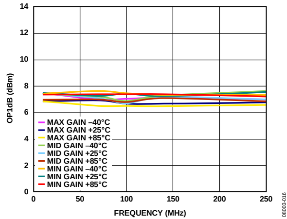
Figure 7. Output P1dB (OP1dB) vs. Frequency at A_V = 6\text{ dB} , A_V = 12\text{ dB} , and A_V = 15.5\text{ dB} over Temperature, 1 k \Omega Differential Load
