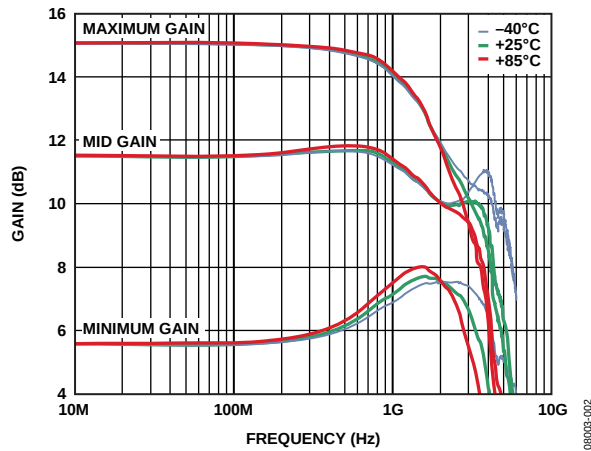
Figure 3. Gain vs. Frequency Response for 200 \Omega Differential Load, A_V = 6\text{ dB} , A_V = 12\text{ dB} , and A_V = 15.5\text{ dB} over Temperature
