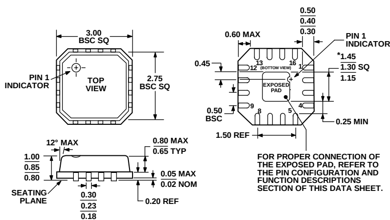
Figure 48. 16-Lead Lead Frame Chip Scale Package [LFCSP_VQ] 3 mm × 3 mm Body, Very Thin Quad (CP-16-2) Dimensions shown in millimeters
