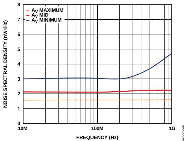
Figure 8. Noise Spectral Density vs. Frequency at A_V = 6\text{ dB} , A_V = 12\text{ dB} , and A_V = 15.5\text{ dB}
