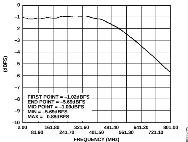
Figure 41. Measured Frequency Response of the Wideband ADC Interface Depicted in Figure 39
