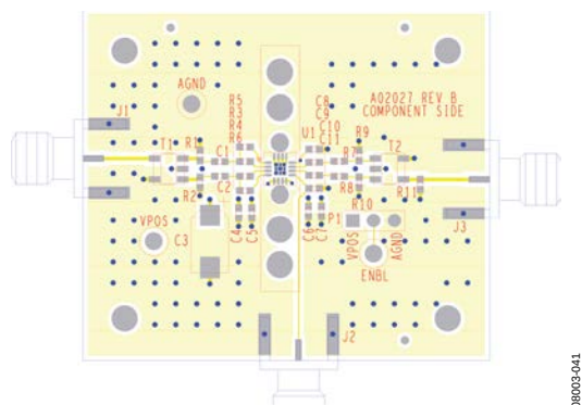
Figure 46. Layout of Evaluation Board, Component Side
