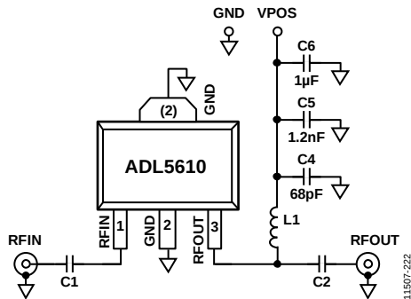
Figure 26. Basic Connections
