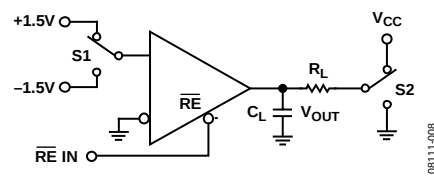
Figure 28. Receiver Enable/Disable
