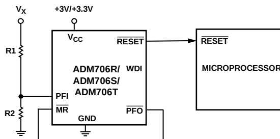
Figure 22. Monitoring 3 V/3.3 V and an Additional Supply, V_x
