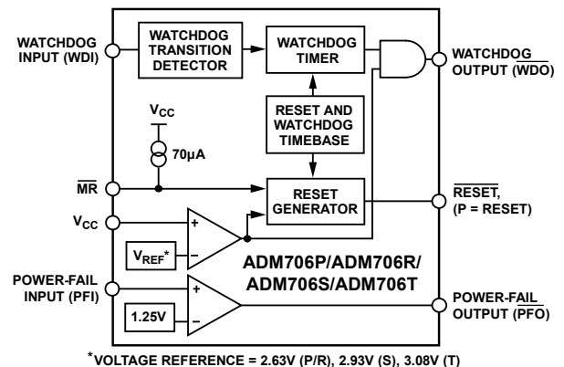
Figure 1. ADM706P/ADM706R/ADM706S/ADM706T
