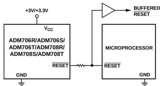
Figure 23. Bidirectional Input/Output RESET
