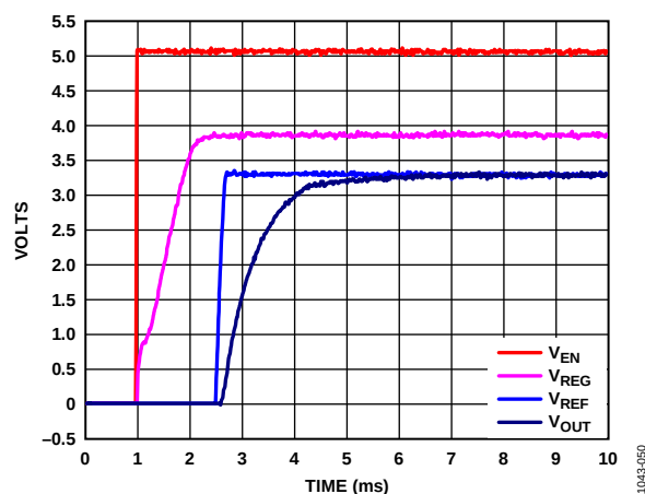
Figure 50. V_{OUT} , V_{REF} , V_{REG} Start-Up Time After V_{EN} Rising, V_{OUT} = 3.3\text{ V} , V_{IN} = 5\text{ V}
