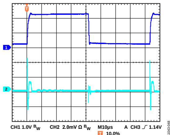
Figure 48. Line Transient Response, 2 V Input Step, I_{LOAD} = 800\text{ mA} , V_{OUT} = 3.3\text{ V} , V_{IN} = 4.5\text{ V} , CH1 = V_{IN} , CH2 = V_{OUT}
