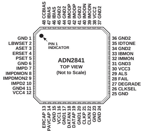
Figure 3. Pin Configuration, 48-Lead LFCSP
