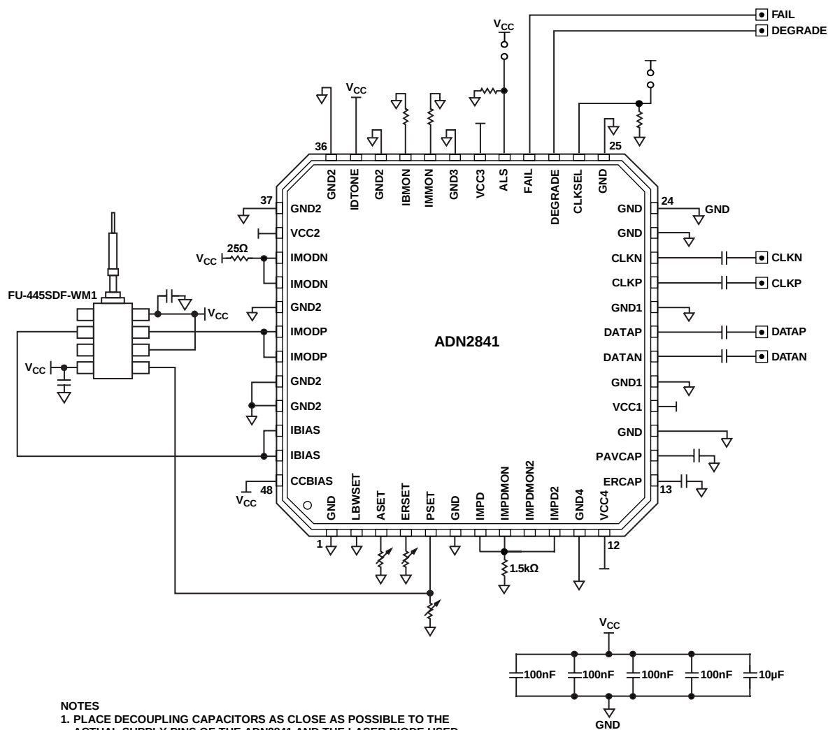
Figure 11. 2.7 Gbps Test Circuit, DC-Coupled, Data Not Clocked, Fast Loop Time Constant Selected
