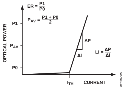
Figure 7. Laser Transfer Function
