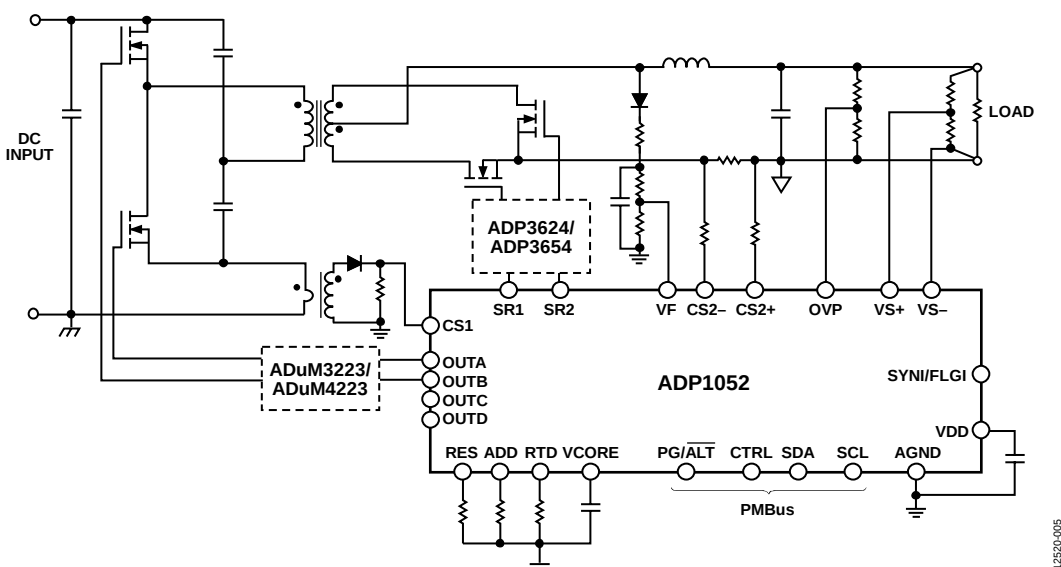
Figure 44. Half Bridge Converter
