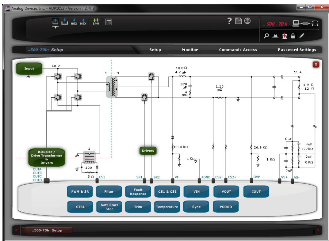
Figure 61. GUI Software
