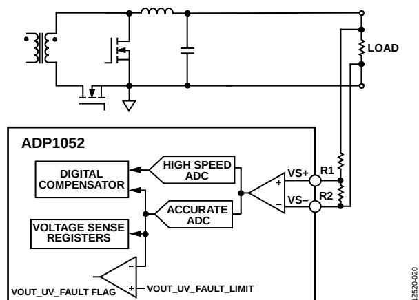
Figure 20. Voltage Sense Configuration
