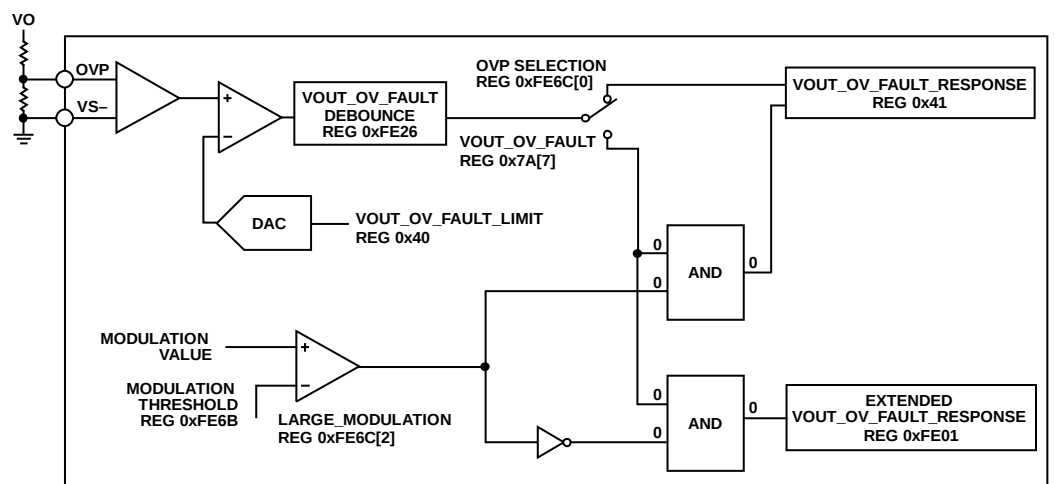
Figure 38. V_{OUT} Overvoltage Protection Circuit Implementation
