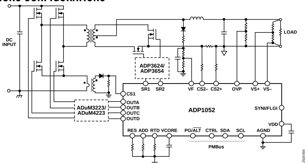
Figure 43. Full Bridge Converter
