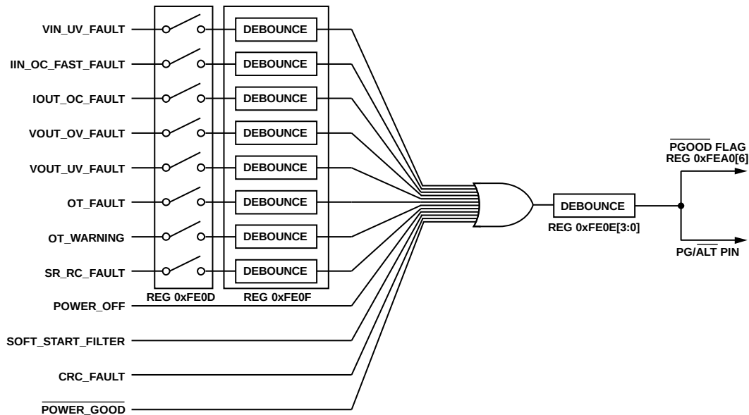
Figure 30. PGOOD Programming
