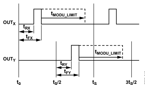
Figure 14. Setting Modulation Limits
