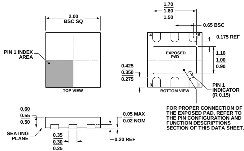
Figure 55. 6-Lead Lead Frame Chip Scale Package [FCSP_UD] 2.00 mm×2.00 mm Body, Ultra Thin, Dual Lead (CP-6-3) Dimensions shown in millimeters
