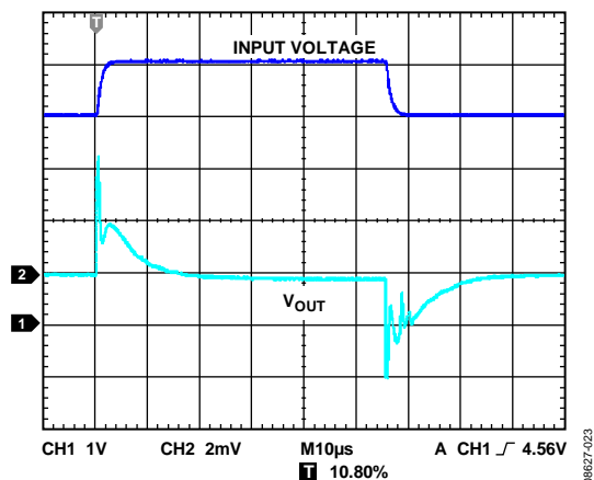
Figure 25. Line Transient Response, C_{IN}, C_{OUT} = 1\text{ }\mu\text{F} , I_{LOAD} = 200\text{ mA}
