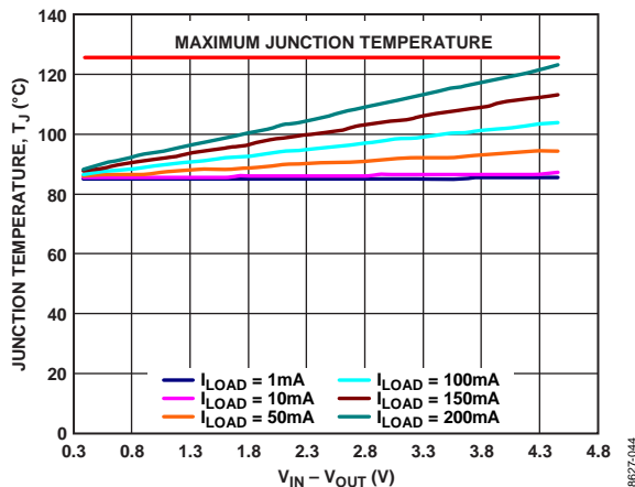
Figure 58. TSOT, T_A = 85^\circ\text{C}
