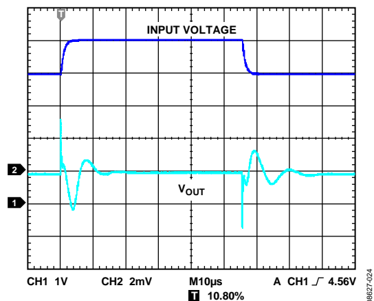
Figure 26. Line Transient Response, C_{IN}, C_{OUT} = 1\text{ }\mu\text{F} , I_{LOAD} = 1\text{ mA}
