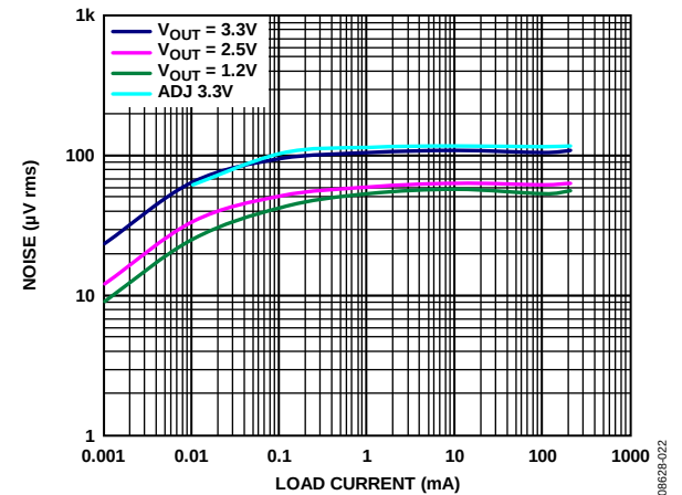
Figure 24. Output Noise vs. Load Current and Output Voltage, V_{IN} = 5\text{ V} , C_{OUT} = 1\text{ µF}
