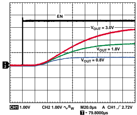
Figure 32. Typical Start-Up Time
