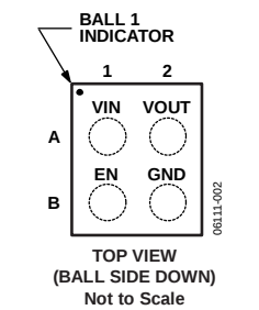
Figure 2. Pin Configuration
