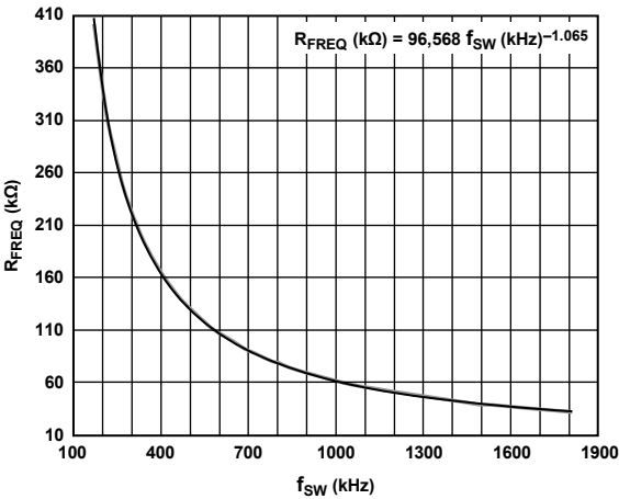
Figure 23. R_{FREQ} VS. f_{SW}
