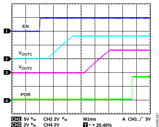
Figure 27. Soft Start with Full Load
