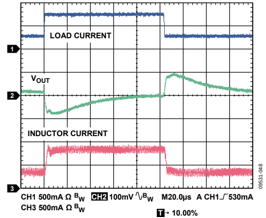
Figure 48. Load Transient, V_{\text{OUT}} = 5 \text{ V} , 300 mA to 800 mA, Load Current Rise Time = 200 ns, V_{\text{IN}} = 8 \text{ V}
