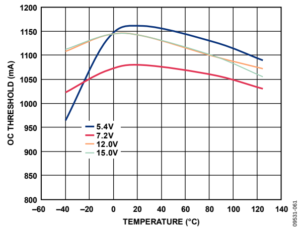
Figure 61. Overcurrent Limit vs. Temperature, V_{OUT} = 5\text{ V} , Different Input Voltages
