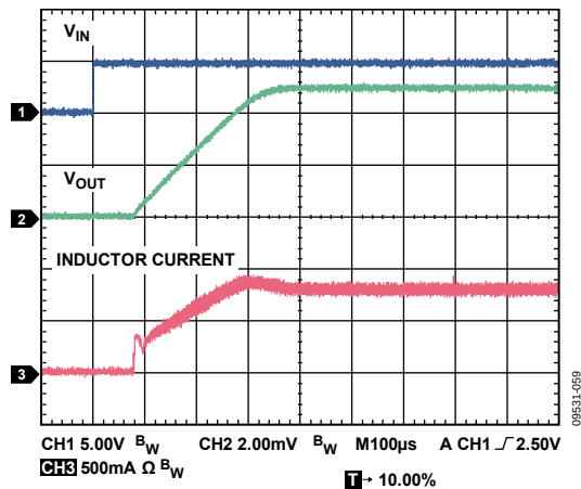
Figure 59. Startup, V_{OUT} = 5\text{ V} , 800 mA, V_{IN} = 7\text{ V}
