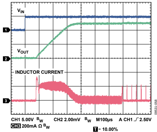
Figure 58. Startup, V_{OUT} = 5\text{ V} , 10 mA, V_{IN} = 7\text{ V}
