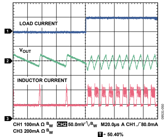
Figure 50. Load Transient, V_{\text{OUT}} = 5 \text{ V} , 10 mA to 110 mA, Load Current Rise Time = 200 ns, V_{\text{IN}} = 8 \text{ V}
