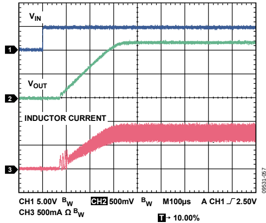
Figure 57. Startup, V_{OUT} = 1.2\text{ V} , 800 mA, V_{IN} = 5\text{ V}
