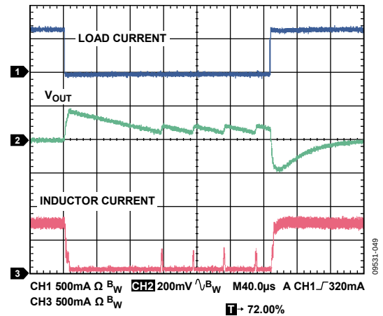
Figure 49. Load Transient, V_{\text{OUT}} = 5 \text{ V} , 1 mA to 800 mA, Load Current Rise Time = 200 ns, V_{\text{IN}} = 8 \text{ V}
