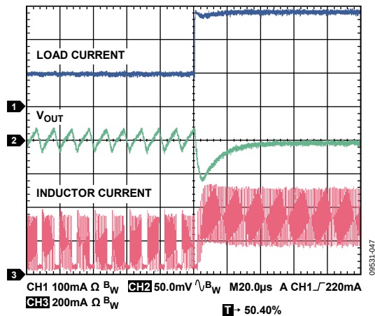
Figure 47. Load Transient, V_{\text{OUT}} = 1.2 \text{ V} , 100 mA to 300 mA, Load Current Rise Time = 200 ns, V_{\text{IN}} = 5 \text{ V}
