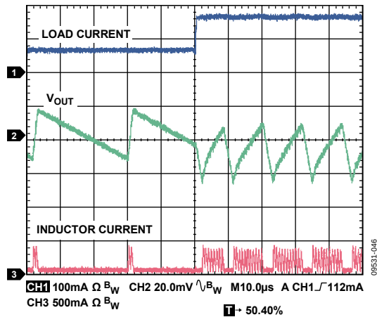
Figure 46. Load Transient, V_{\text{OUT}} = 1.2 \text{ V} , 10 mA to 110 mA, Load Current Rise Time = 200 ns, V_{\text{IN}} = 5 \text{ V}
