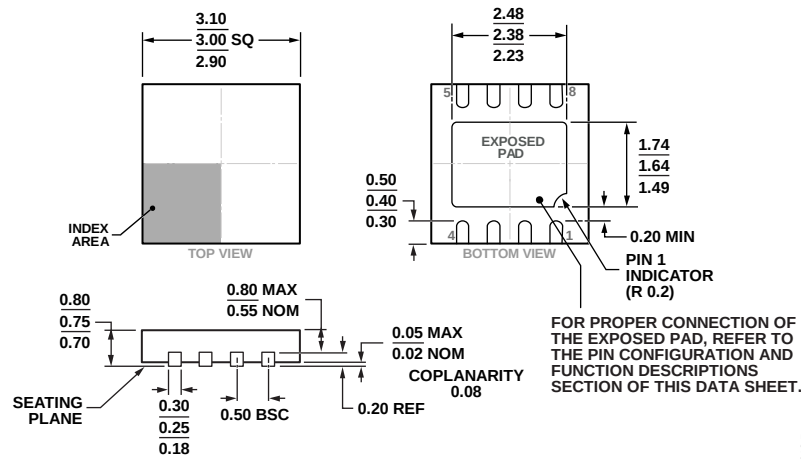
Figure 93. 8-Lead Lead Frame Chip Scale Package [LFCSP_WD] 3 mm × 3 mm Body, Very Very Thin, Dual Lead (CP-8-5)
