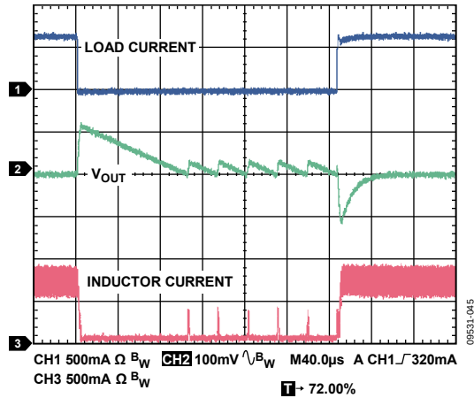
Figure 45. Load Transient, V_{\text{OUT}} = 1.2 \text{ V} , 10 mA to 800 mA, Load Current Rise Time = 200 ns, V_{\text{IN}} = 5 \text{ V}
