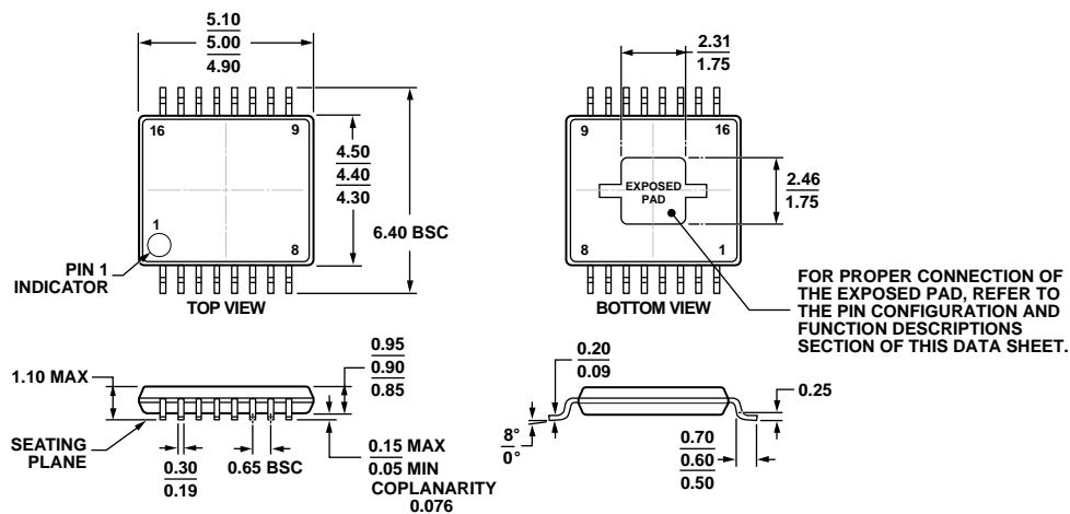
Figure 42. 16-Lead Thin Shrink Small Outline with Exposed Pad [TSSOP_EP] (RE-16-3)
