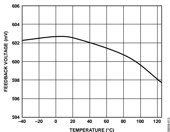
Figure 14. FB Voltage vs. Temperature
