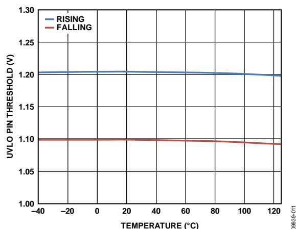
Figure 13. UVLO Pin Threshold vs. Temperature
