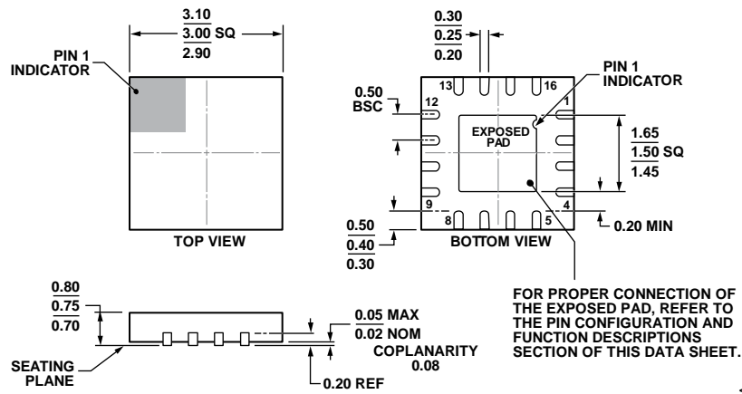
Figure 64. 16-Lead Lead Frame Chip Scale Package [LFCSP_WQ] 3 mm x 3 mm Body, Very, Very Thin Quad (CP-16-27) Dimensions shown in millimeters
