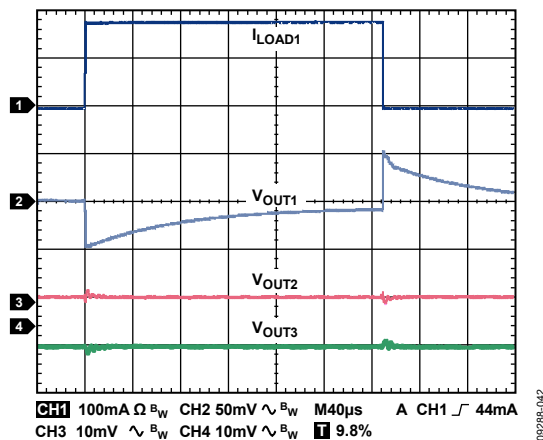
Figure 51. Output Transient Response, I_{LOAD1} = 1\text{ mA to }200\text{ mA} , I_{LOAD2} = 1\text{ mA} , I_{LOAD3} = 1\text{ mA} , CH1 = I_{LOAD1} , CH2 = V_{OUT1} , CH3 = V_{OUT2} , CH4 = V_{OUT3}
