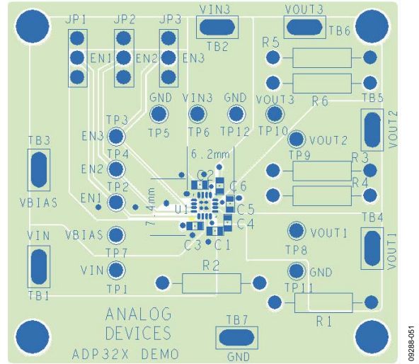
Figure 62. Example of PCB Layout, Top Side
