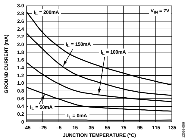
Figure 9. Ground Current vs. Junction Temperature
