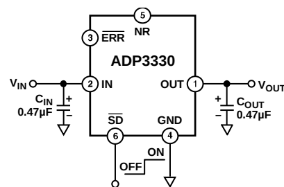
Figure 2. Typical Application Circuit
