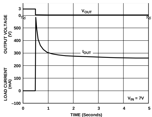
Figure 17. Short-Circuit Current
