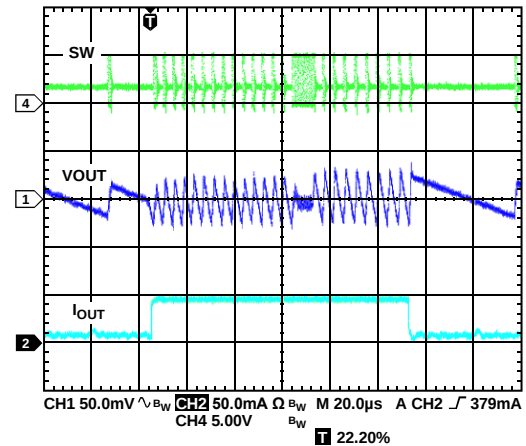
Figure 26. BUCK2 Response to Load Transient, I_{OUT2} from 1\text{ mA} to 50\text{ mA} , V_{OUT2} = 1.8\text{ V} , Automatic Mode
