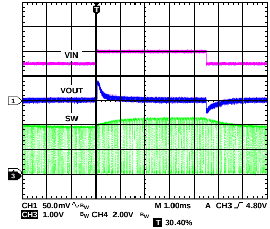
Figure 24. Buck2 Response to Line Transient, V_{IN} = 4.5\text{ V} to 5.0\text{ V} , V_{OUT2} = 1.8\text{ V} , PWM Mode
