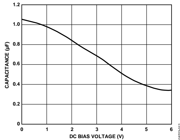
Figure 52. Capacitance vs. Voltage Characteristic
